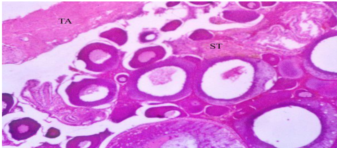
Fig. 5: Section of catfish's ovary during winter showing, very thick tunica albuginea (TA) and increased stromal connective tissue (ST)
