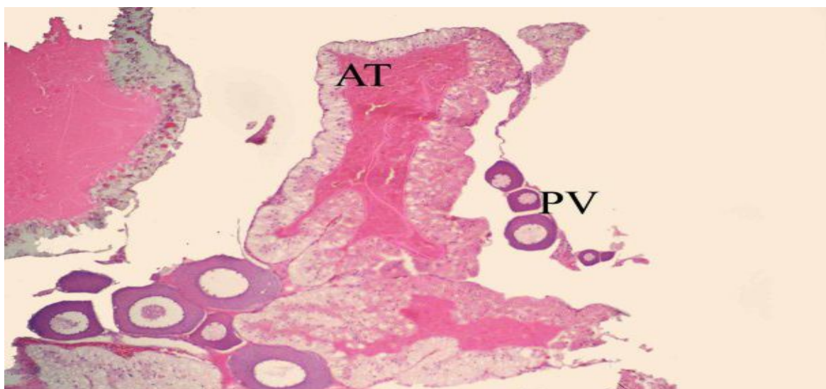
Fig. 8: Section of catfish's ovary during autumn showing, predominance of atretic (AT) and pre-vitellogenic follicles (PV).
