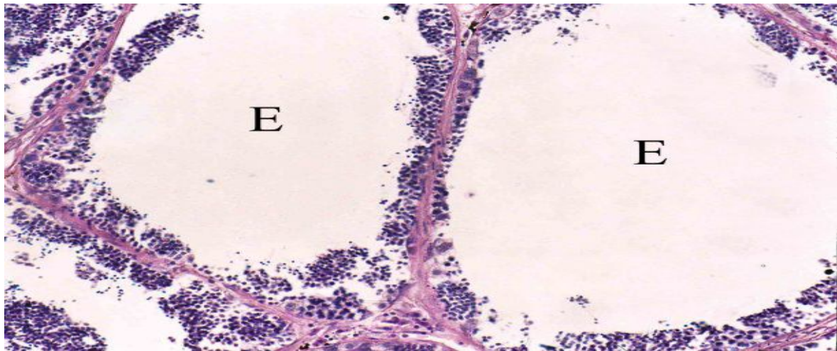
Fig. 4: Section of catfish's testis during autumn showing, empty testicular lobules (E). Notice all developmental stages; spermatogonia (arrow), spermatocytes cyst (SC), spermatid cyst (ST). PAS technique ( \times 200 )
