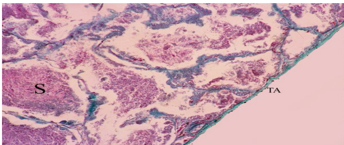
Fig. 3: Section of catfish's testis during summer showing, thin tunica albuginea (TA) compared to Figure 1. Testicular lobules are filled with spermatozoa (S). Crossman's trichrome ( \times 100 )
