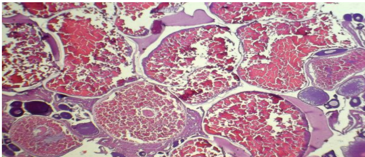
Fig. 7: Section of catfish's ovary during summer showing, abundant mature follicles (MF)
