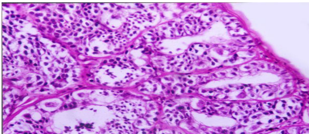
Fig. 2: Section of catfish's testis during spring showing testicular lobules filled with all spermatogenic cells. H&E ( \times 200 )
