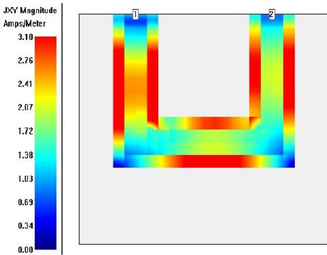
Fig. 3: U-Patch shaped with current distribution and feed points
