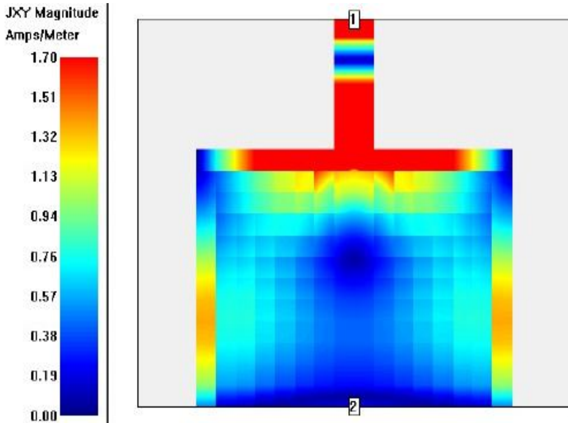
Fig. 2: Rectangular Patch shape with Current distribution and feed points
