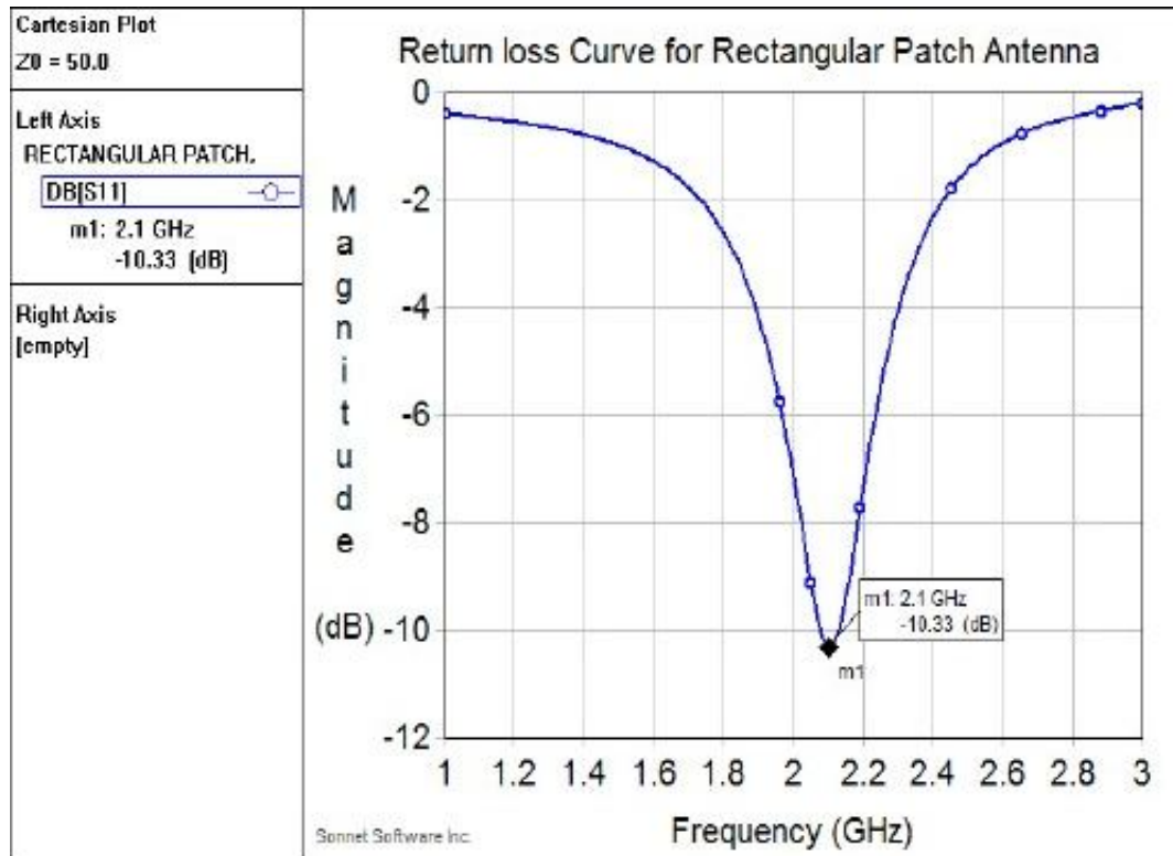
Fig. 4: Simulated Return Loss of rectangular microstrip patch antenna
